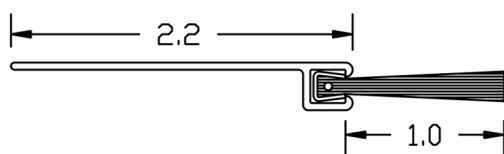
C002.2 W/ 1.5" BRUSH
